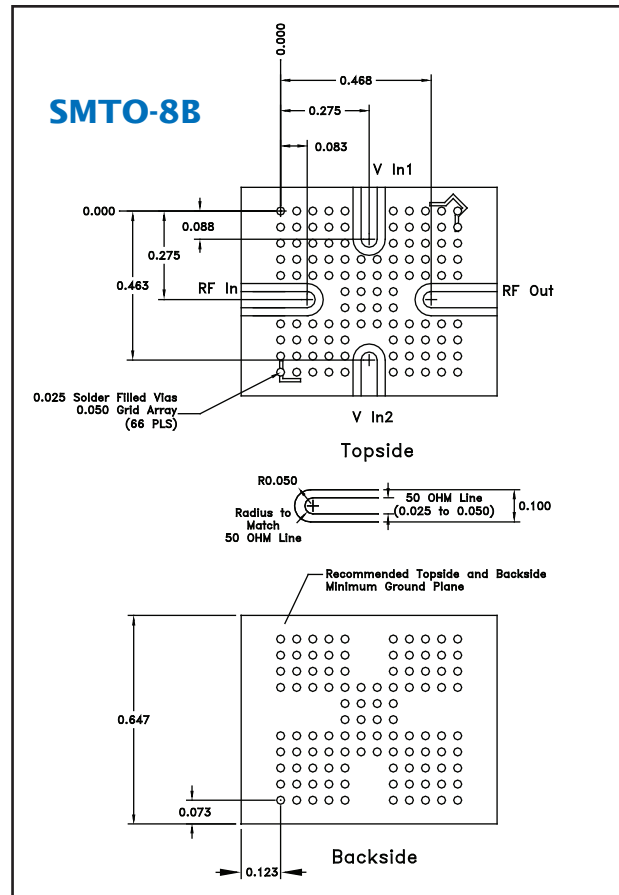
FIGURE 2. Recommended mounting layout for surface mount packages (SMT0-8B).
