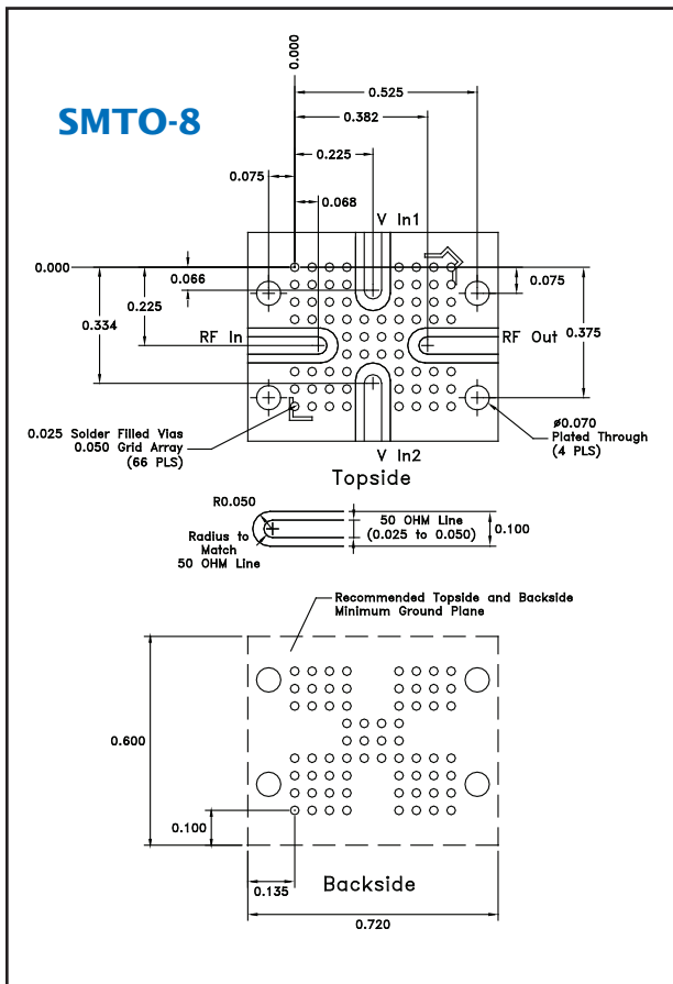
FIGURE 1. Recommended mounting layout for surface mount packages (SMT0-8).
